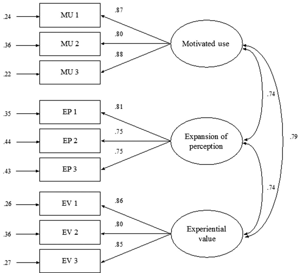
Figure 1 — Latent factor solution for the ToRQ with completely standardized \lambda loadings, \chi^2(24) = 55.31, p < .001 , NNFI = .973, CFI = .982, SRMR = .027, RMSEA = .065 (90% confidence interval [.043, .089], p = .0125 ). Note. MU = motivated use; EP = expansion of perception; EV = experiential value; ToRQ = Transfer of Responsibility Questionnaire; NNFI = nonnormed fit index; CFI = comparative-fit index; SRMR = standardized root mean square residual; RMSEA = root mean square error of approximation.
